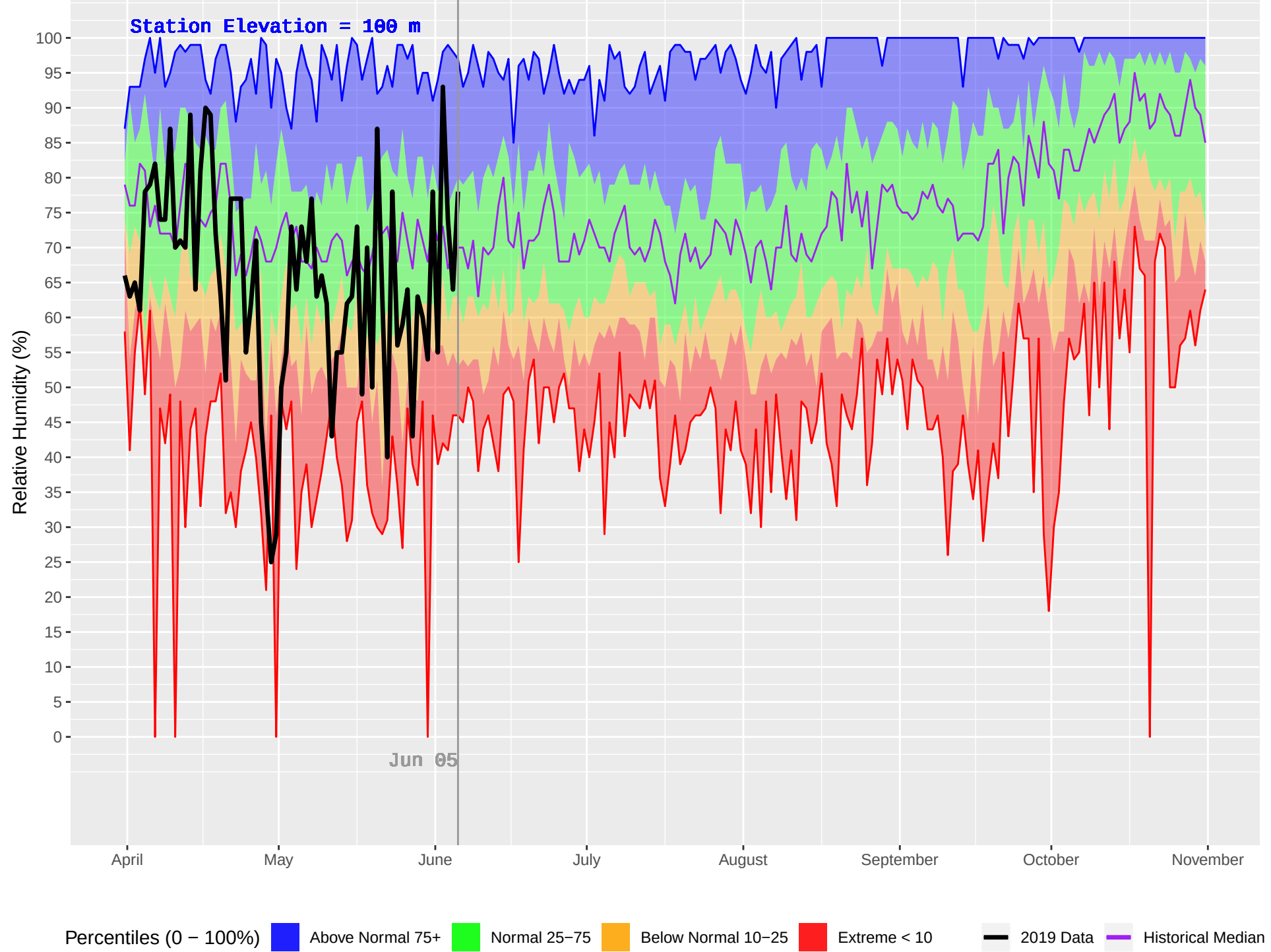
HONNA (93) : Historical (1986–2018) and Current (2019) Daily Relative Humidity
