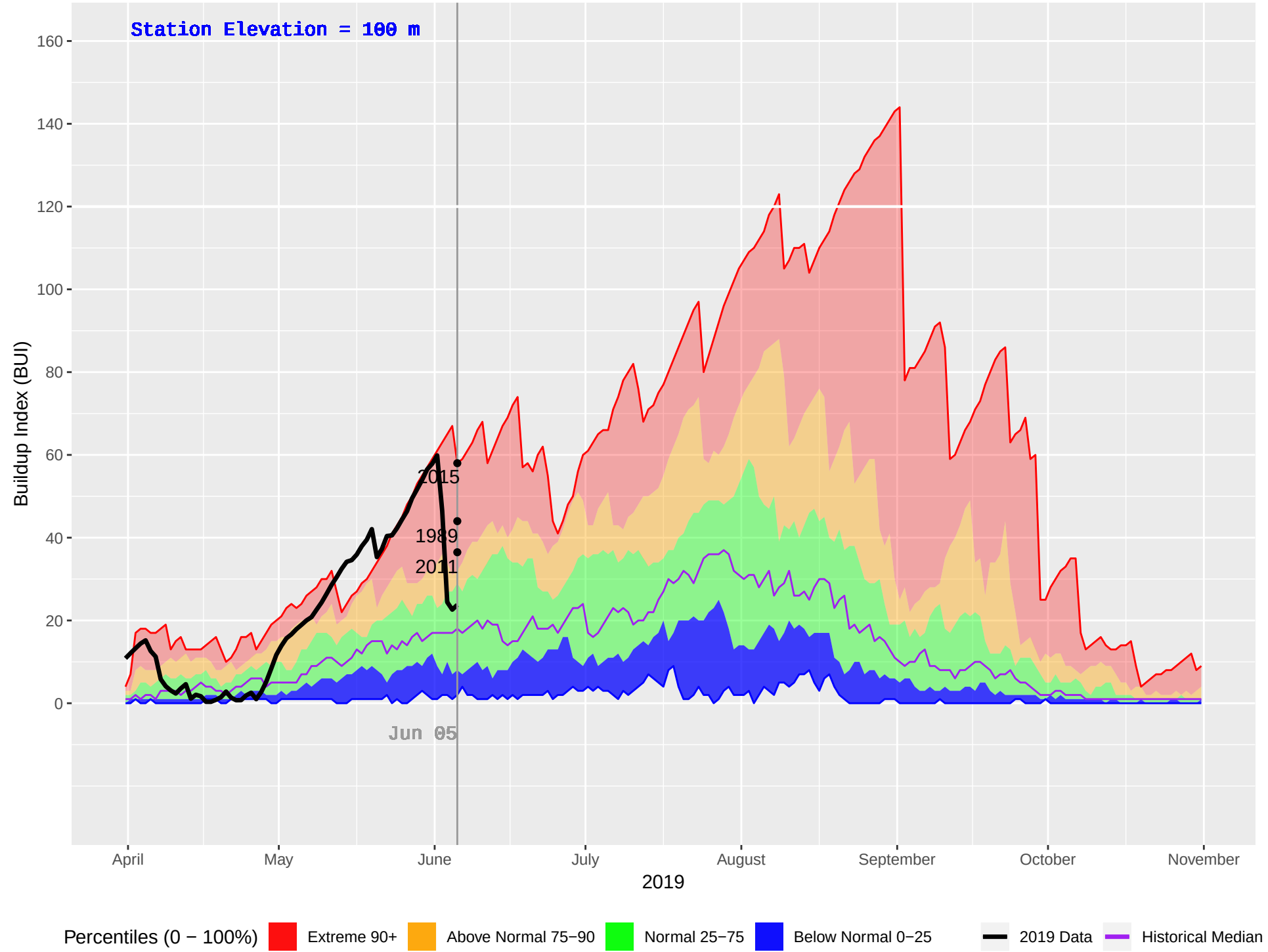
HONNA (93) : Historical (1986–2018), Current (2019) Daily Buildup Index (BUI)
