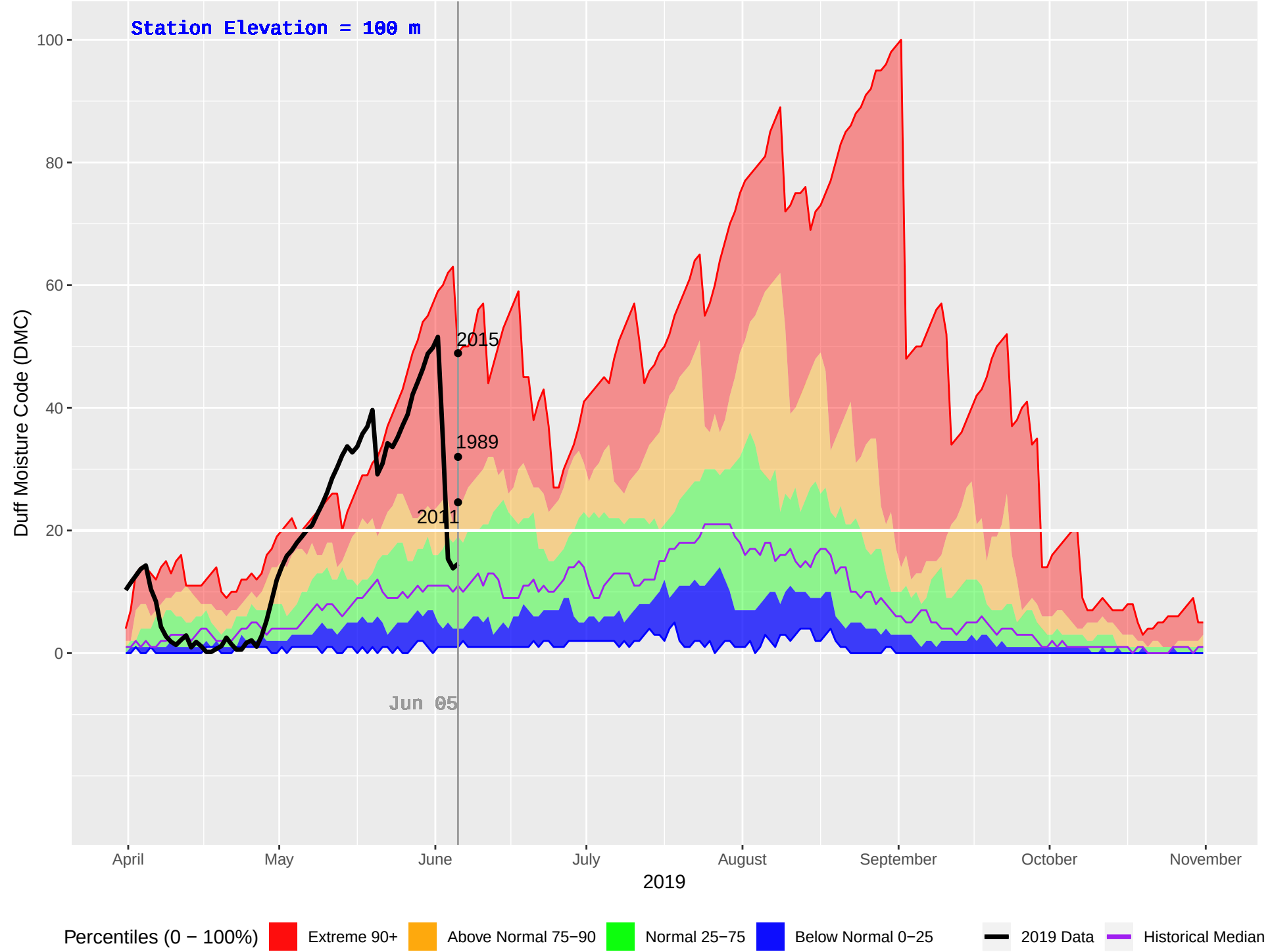
HONNA (93) : Historical (1986–2018), Current (2019) Daily Duff Moisture Code (DMC)
