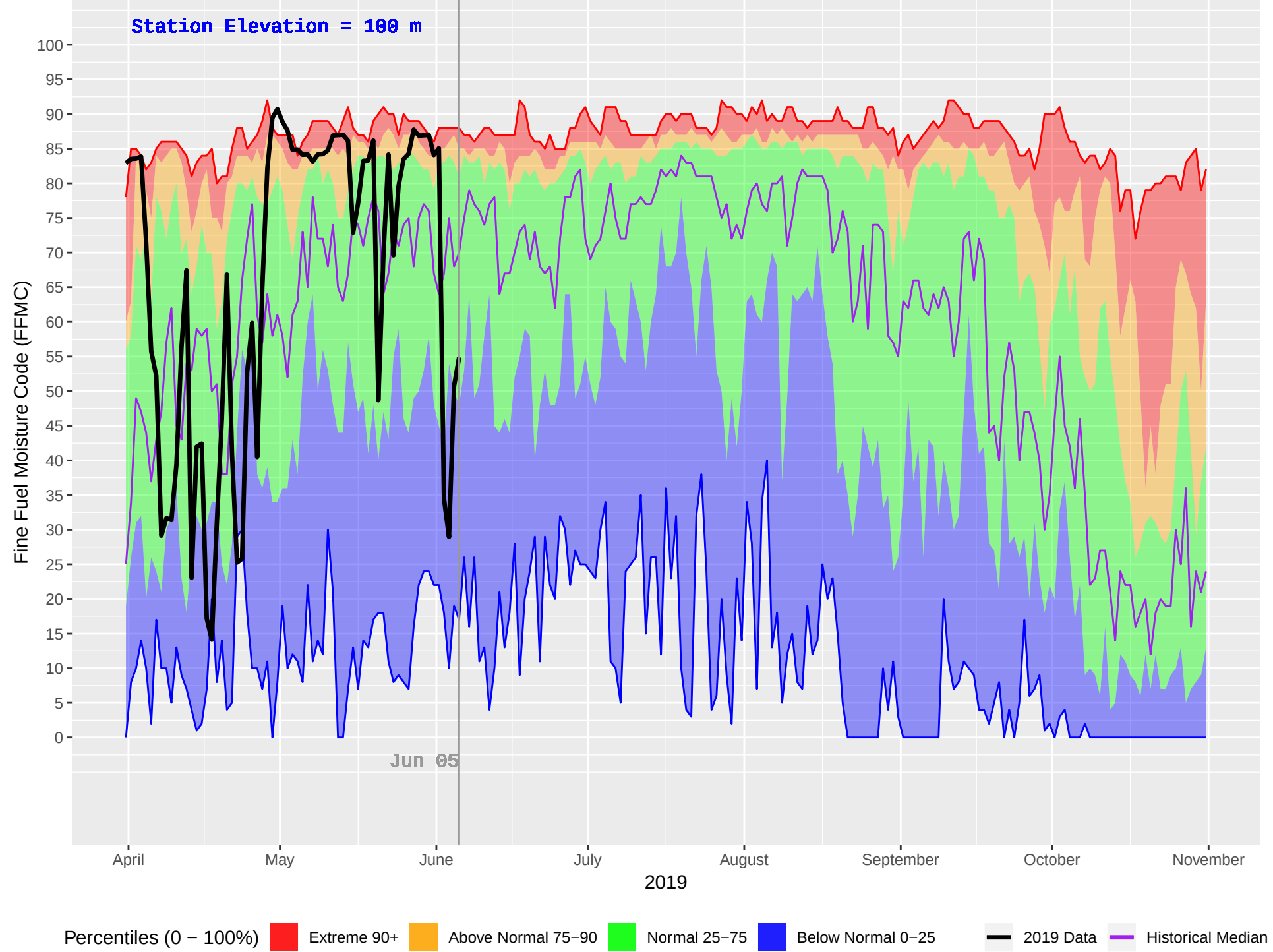
HONNA (93) : Historical (1986–2018) and Current (2019) Daily Fine Fuel Moisture Code (FFMC)
