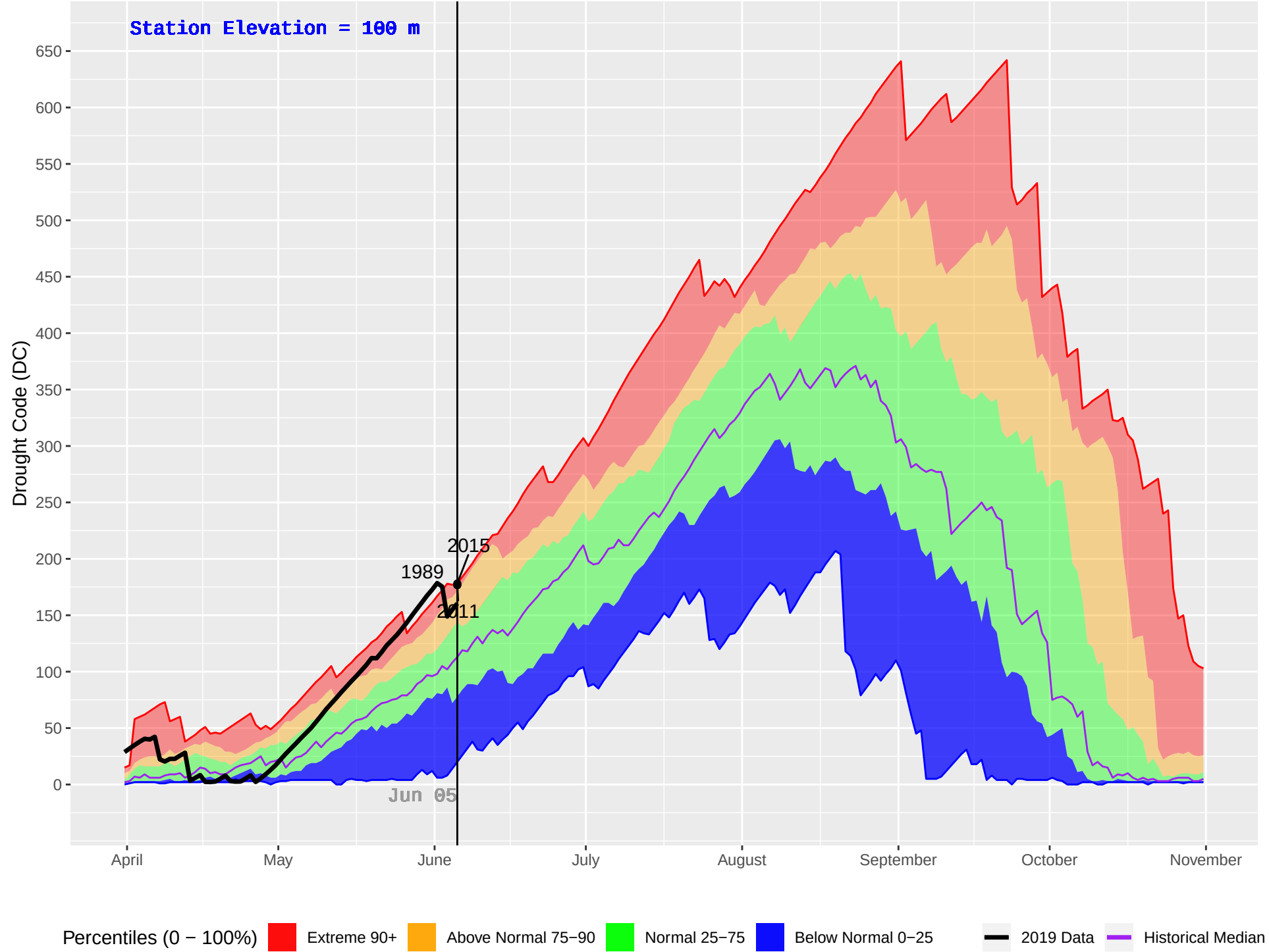
HONNA (93) : Historical (1986–2018) and Current (2019) Daily Drought Code (DC)
